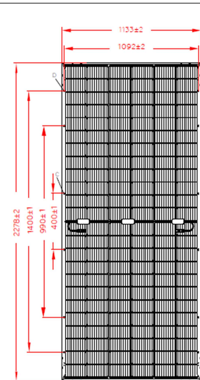
Mechanical Drawings of PV Module (Gen 2) ASB-M10-144-XXX
