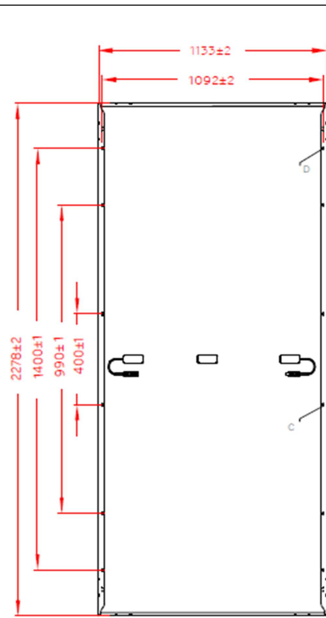
Mechanical Drawings of PV Module (Gen 2) ASM-M10-144-XXX
